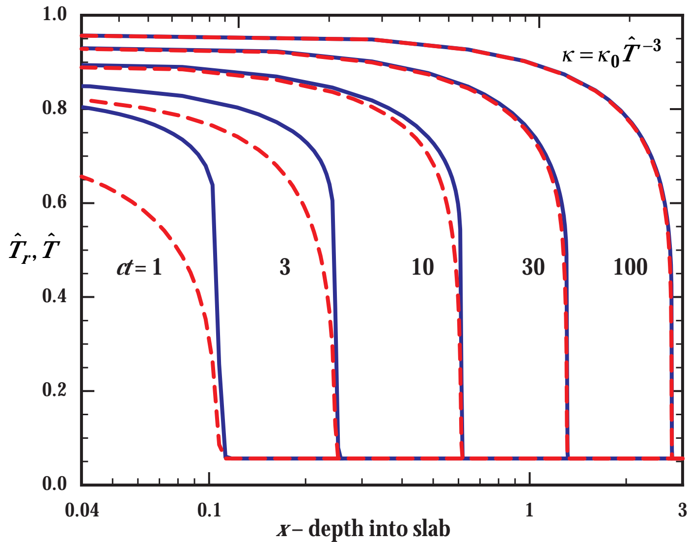
Figure 8. The normalized radiation (solid lines) and material (dashed lines) temperatures are shown as a function of space at different times for the temperature-dependent opacity problem.
