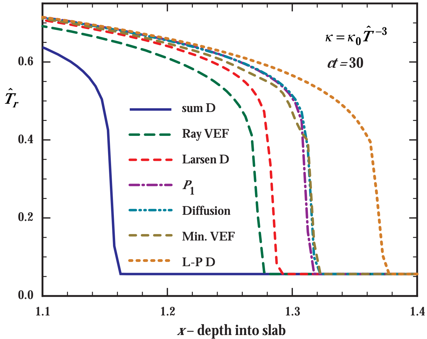
Figure 9. The normalized radiation temperature is shown as a function of space at one time for several different approximate transport models. The models listed top to bottom are in the left to right order at T_r = 0.2 .
