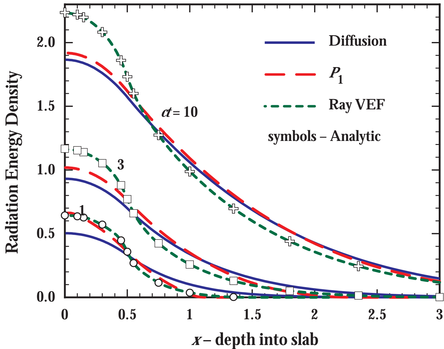
Figure 2. The analytic benchmark solution of Su and Olson, 1 the symbols, is compared to diffusion, P_1 , and a characteristics ray Eddington factor solutions on a linear scale.
