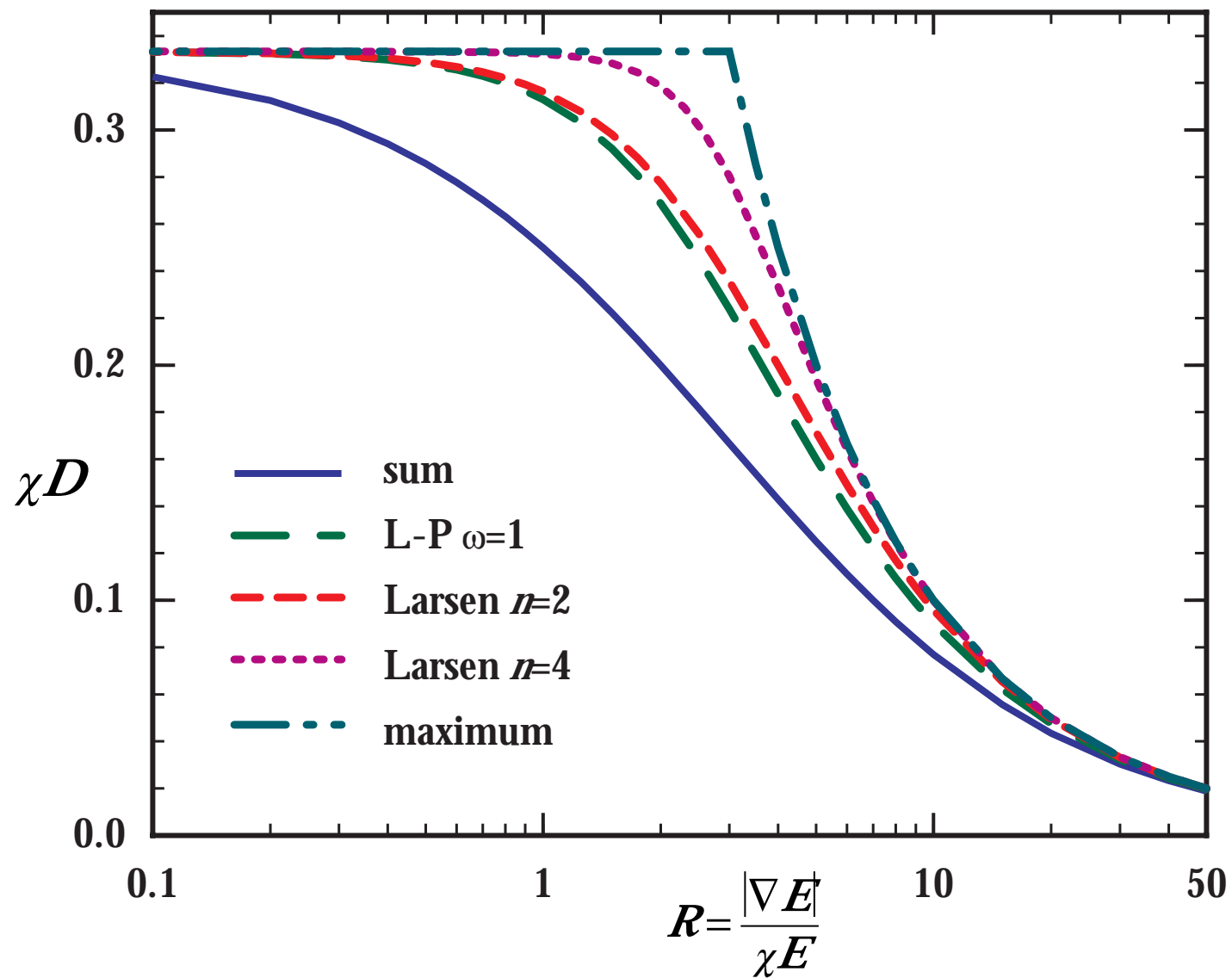
Figure 1. The scaled diffusion coefficient is shown as a function of a scaled energy gradient. The legend listing the models from top to bottom describes the curves from left to right. L-P refers to the Levermore-Pomraning 10 flux limiter.
